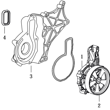
(fig.2) 20411832 Water Pump Pulley Ø168mm
