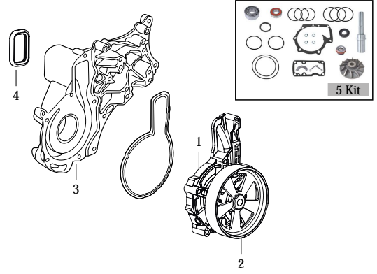
(fig.2) 3161498 Water Pump Pulley Ø140mm
