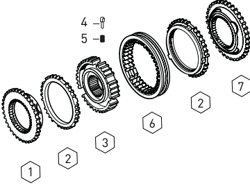
SYNCHRONIZER KIT 5th/6th
