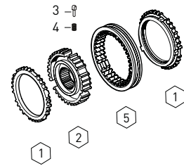
SYNCHRONIZER KIT 1st/2nd
