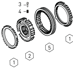
SYNCHRONIZER KIT 3rd/4th
