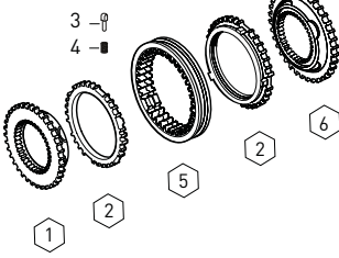
SYNCHRONIZER KIT 5th/6th
