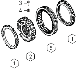
SYNCHRONIZER KIT 5th/6th
